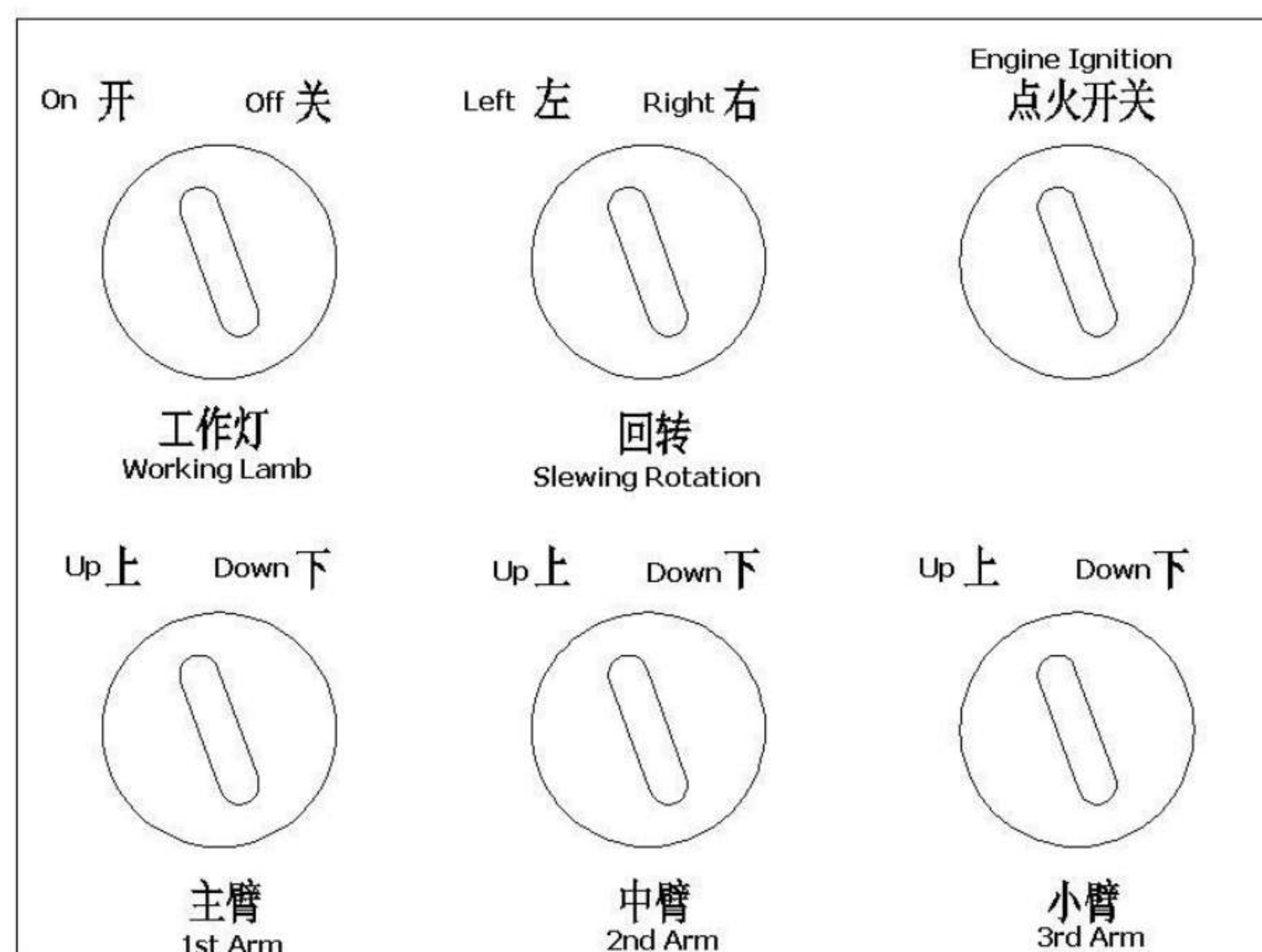
Technical Drawing
